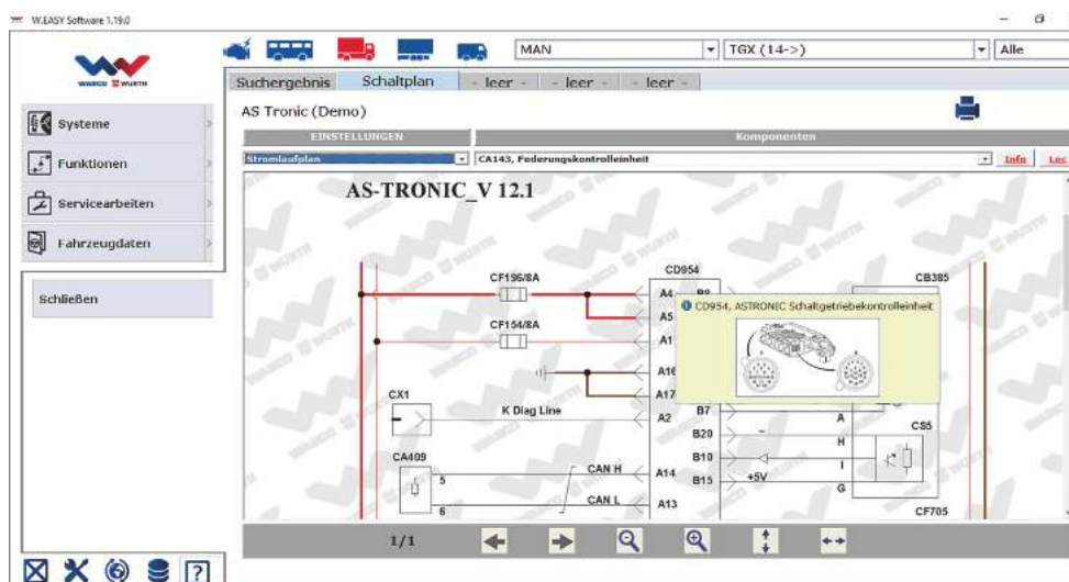
Interactive circuit diagrams
